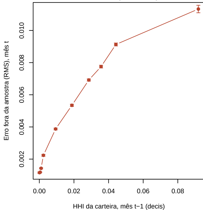
B) Defasada (t-1 -> t) corr=0.49 (N=36.887)
